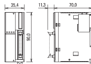
FC4A-D20K3, FC4A-D20S3
